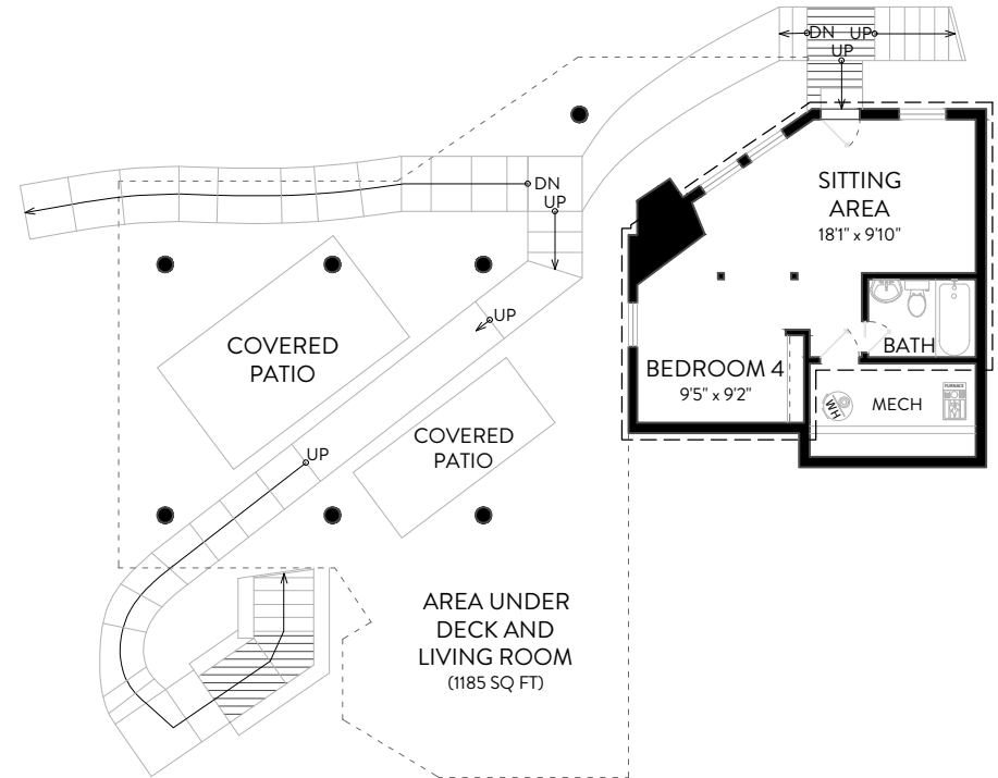
LOWER LEVEL 375 SQ FT
